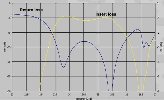
25GHz Phase Shifter
