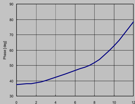
25GHz Phase shifter Phase
