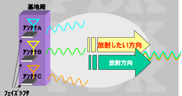
25GHz Phase Shifter
